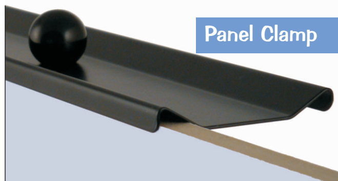
Above: Panel Clamp holding 10mm foamcore display board.
